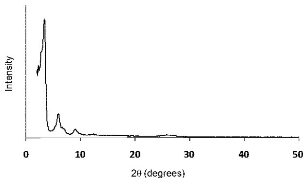
Figure 2. Powder diffraction pattern for COF-5 produced by microwave technique.
