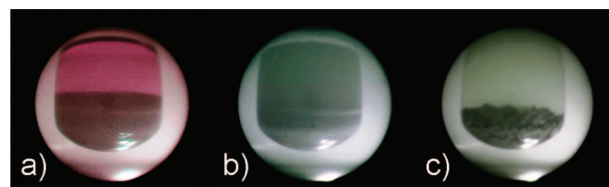
Figure 1. Digital camera images recorded from the observation port of the microwave reactor showing COF-5 reaction and purification: (a) gray-purple COF-5 powder formed after initial synthesis; (b) removal of trapped HHTP-oxidation impurities by microwave extraction process (acetone); (c) second microwave extraction results in purified gray COF-5 powder ( S_{\text{BET}} = 2019 m 2 g −1 ).
